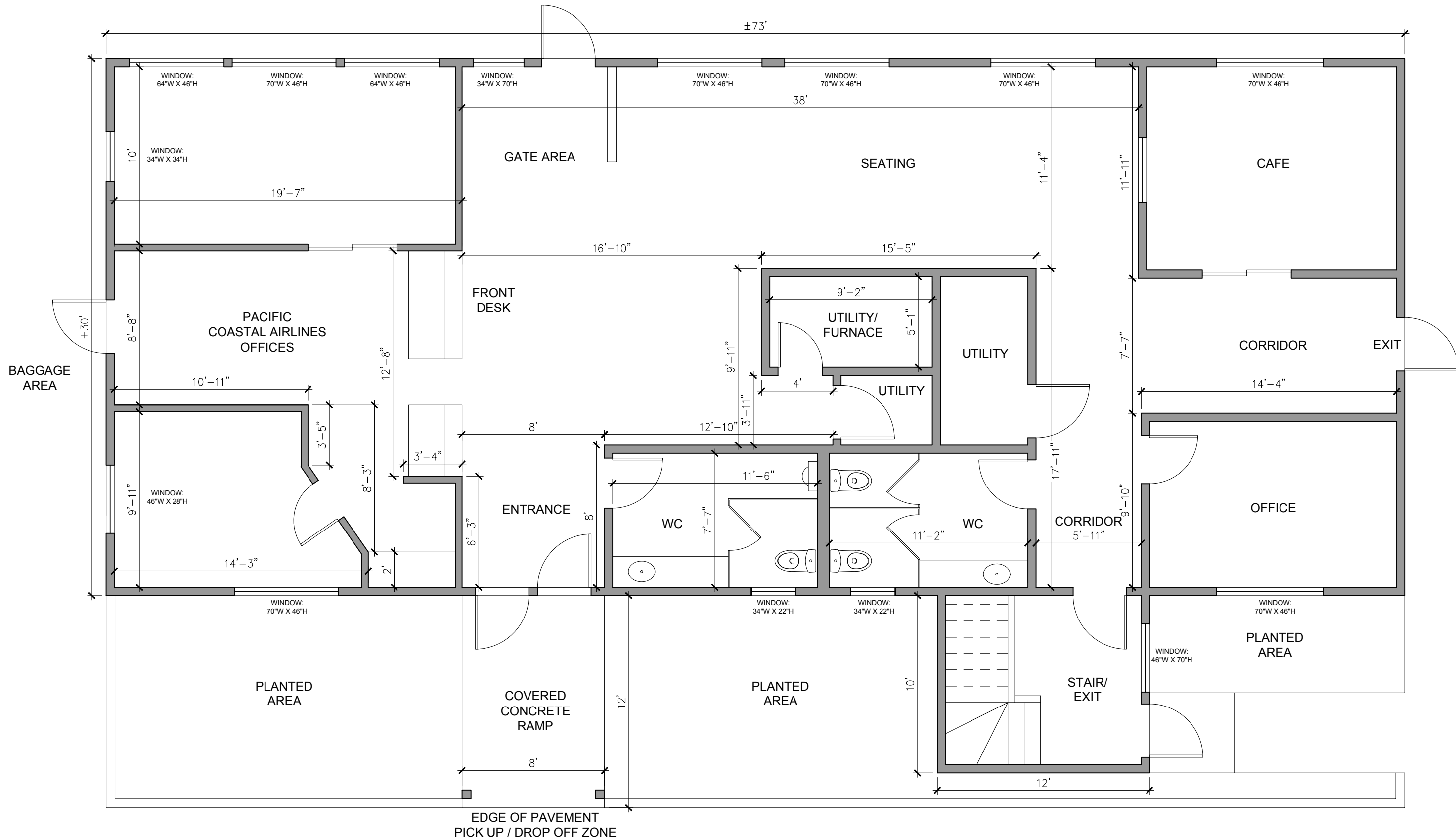
BELLA COOLA AIRPORT TERMINAL - EXISTING GROUND FLOOR PLAN *MEASUREMENTS ARE APPROXIMATE* SCALE: \frac{3}{16}" = 1'-0"
